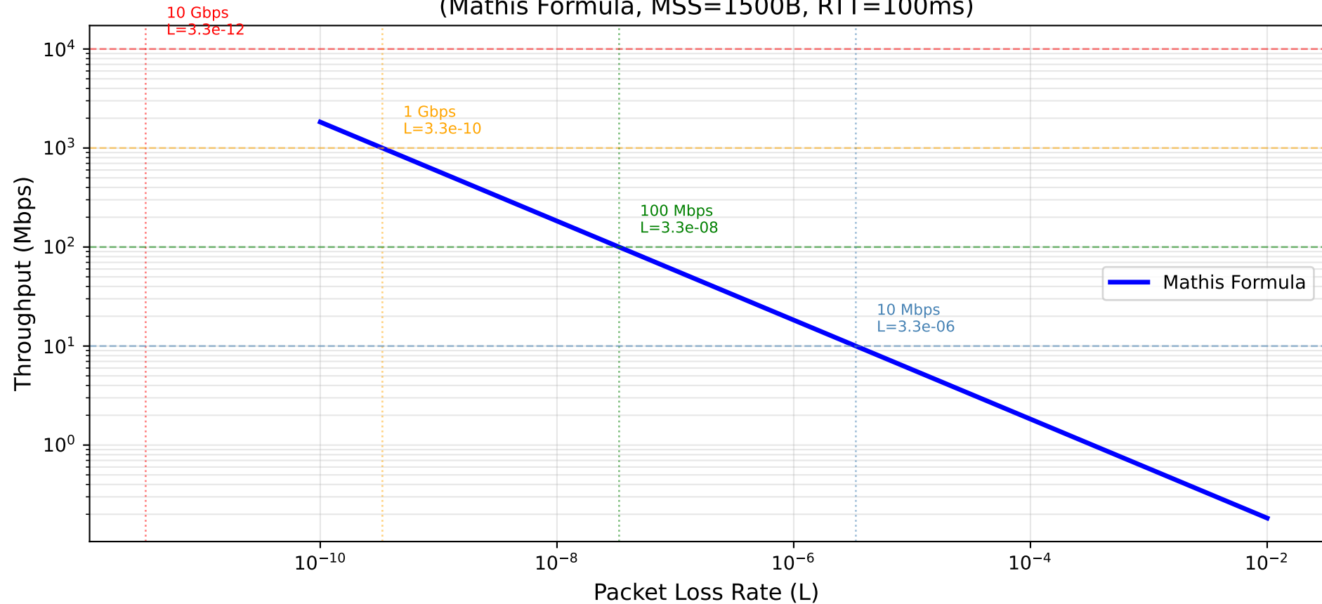
TCP Throughput vs. Loss Rate (Mathis Formula, MSS=1500B, RTT=100ms)
